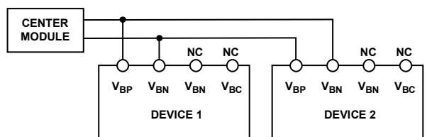
Figure 17. Dual Device—Parallel Configuration
