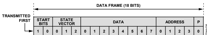
Figure 38. Configuration Mode Transmit Data Frame
